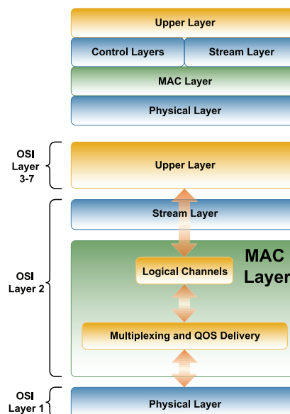
Figure 2: Example of FLO Network
