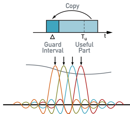
Figure 3: OFDM Symbols
